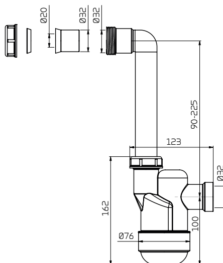
Dimensional drawing (all measurements are in mm).
