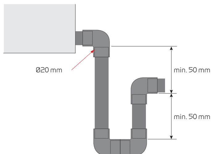
Illustration of connection on the side of the ventilation unit
